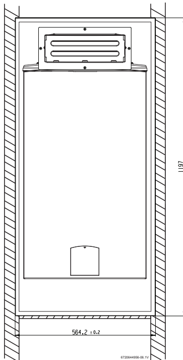
Fig. 11 Mounting the heater inside recess box
