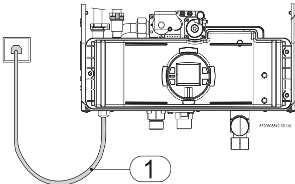
Fig. 22 Connecting power supply cord
